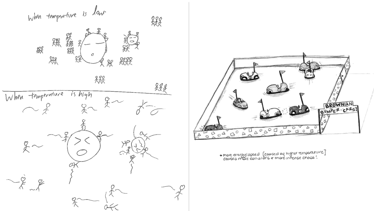
Fig. S2. Drawings created by university students after the instructions, “Draw, as if explaining to a high school student, how the motions of large and small particles suspended in a fluid are affected by an increase in temperature of the fluid.” The two related drawings on the left-hand side demonstrate a greater understanding of concepts such as particle size and motion compared with the picture on the right-hand side. [Image courtesy of Picturing to Learn, funded by NSF DUE-0925110]
