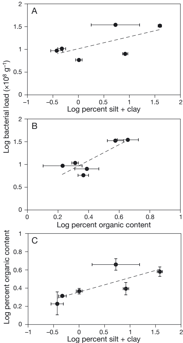
Fig. 4. Covariation (means \pm 1 SE) among (A) sediment bacterial load and percent silt + clay, (B) bacterial load and percent organic content, and (C) percent organic content and percent silt + clay at 6 field sites. Each point represents the average for the site (left to right): (A,C) AL1, FJ, FB, MB, AL2, GB; (B) AL1, FJ, FB, AL2, GB, MB. Dashed lines are best fit from ordinary least squares regression. Error bars may be smaller than the symbols for bacterial load
