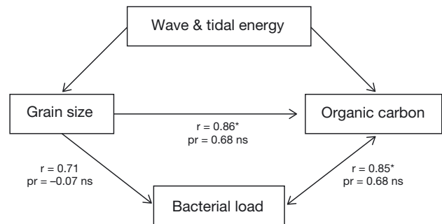
Fig. 5. Functional relationships expected among bacterial load, wave energy, grain size, and organic content in intertidal environments (adapted from Dale 1974). Values beside lines are correlation coefficients ( r ) and partial correlation coefficients ( pr ) calculated for sediment among the 6 habitats surveyed in the present study. *Significant ( p < 0.05 ). ns = not significant
