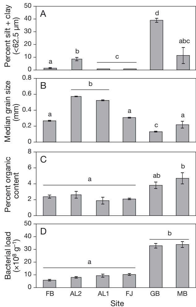
Fig. 3. Sediment characteristics (A: percent silt + clay, B: median grain size, C: percent organic content, D: bacterial load) at the 6 field sites. The sites are arranged from smallest to largest bacterial load. Error bars represent 1 SE. Site abbreviations as in Fig. 1. Bars with different lowercase letters are sites that were significantly different in percent organic content by Tukey multiple comparisons tests and in percent silt + clay, median grain size, and bacterial load by non-parametric multiple comparisons
