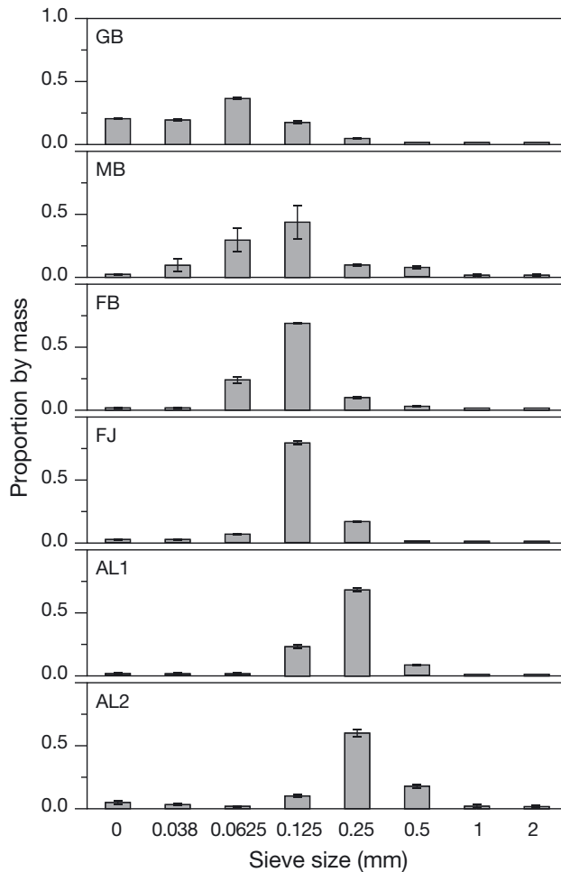
Fig. 2. Proportion (by dry mass) of sediment collected on each sieve size at each study site. Percent silt + clay is the sum of the 2 smallest sieve sizes (<62.5 \mu\text{m} ). Error bars represent 1 SE. Site abbreviations as in Fig. 1
